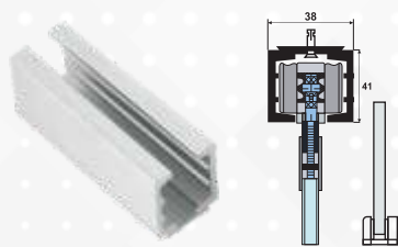
ASL-44-B1 Aluminium Track (Single Door) Available in 8, 10 & 13 Ft.
