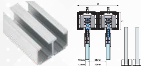
ASL-44-B2 Aluminium Track (Double Door) Available in 8, 10 & 13 Ft.
