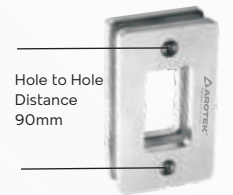
ASL-HN-80 Sliding Handle (Rectangle)
