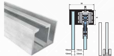
ASL-44-B3 Aluminium Track (Door + Fix Glass) Available in 8, 10 & 13 Ft.
