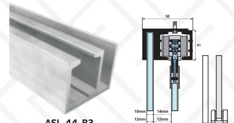
ASL-44-B3 Aluminium Track (Door + Fix Glass) Available in 8, 10 & 13 Ft.
