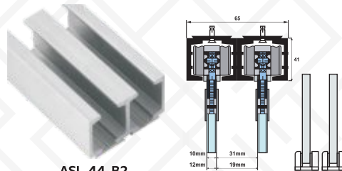
ASL-44-B2 Aluminium Track (Double Door) Available in 8, 10 & 13 Ft.
