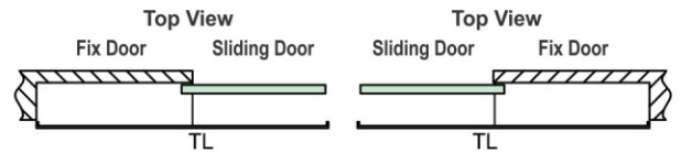
CPSS-104 (Soft Close) Profile Synchronized Sliding System
