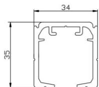
CPTS-104 Top Sliding Track
