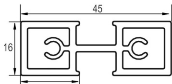
CGP-105 Divider Profile
