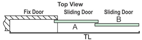
CPSS-101 (Soft Close) Telescopic Sliding System (2 Door)
