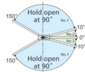
CHFS-100 Hydraulic Floor Hinge
