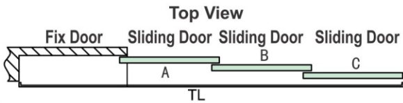
CPSS-102 (Soft Close) Telescopic Sliding System (3 Door)
