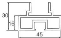
CPTS-106 Top and Bottom Channel
